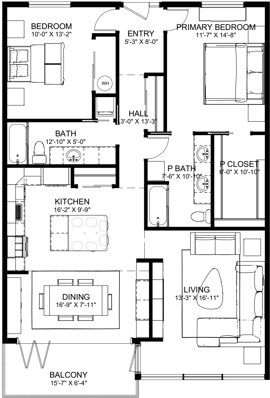
2 BED FLOOR PLAN 1/3"=1'
