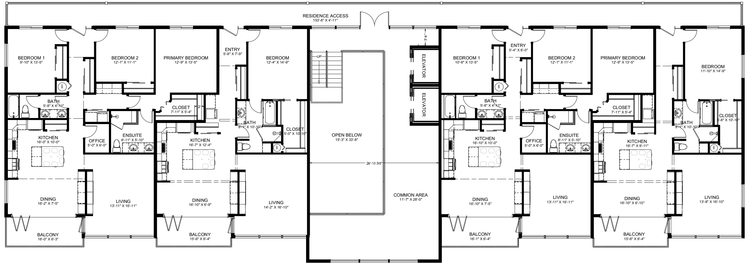
RESIDENTIAL FLOOR 1 & 3 BEDROOM 1/3"=1'
