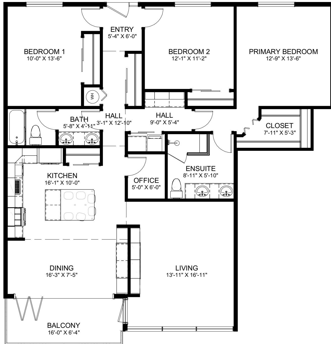
3 & 1 BEDROOM FLOOR PLAN
